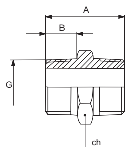
BSPT male / male adaptor
