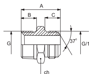
NPT male adaptor / NF-JIC male
