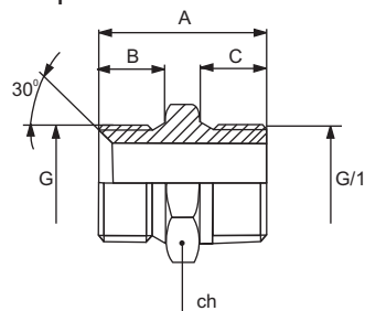
BSP to NPT male / male adaptor
